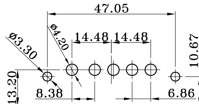
PCB LAYOUT
