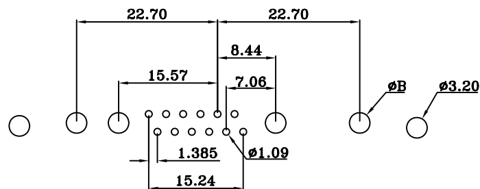
PCB LAYOUT
