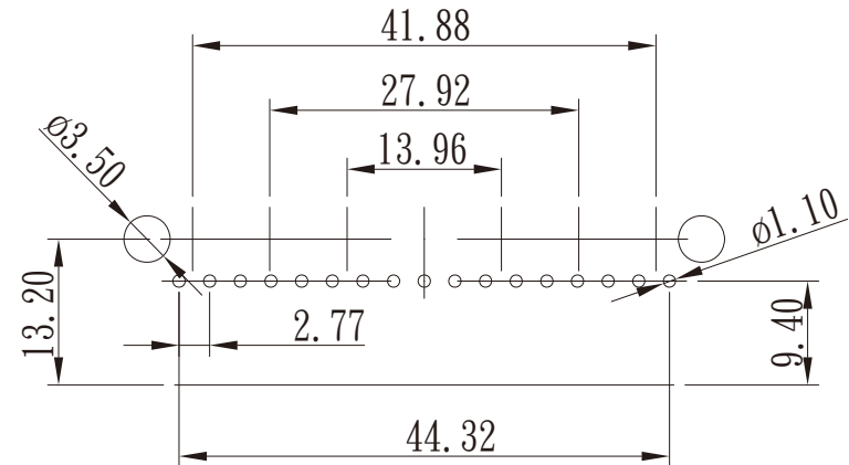
PCB LAYOUT
