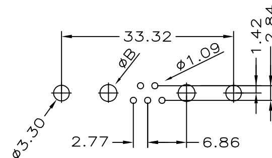
PCB LAYOUT
