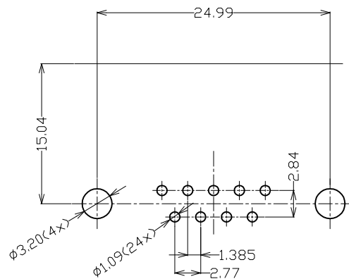
RECOMMEND P.C.B. LAYOUT TOP VIEW
