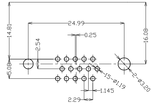
P.C.B. LAYOUT (TOLERANCE ±0.05) TOP VIEW
