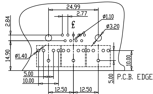
RECOMMENED P.C.B. LAYOUT
