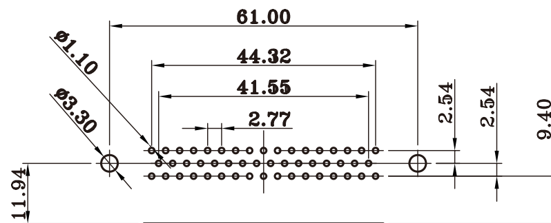
PCB LAYOUT
