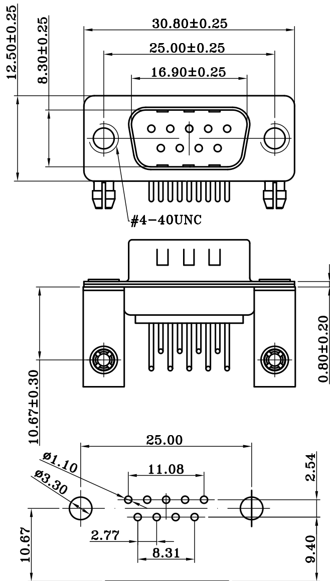
PCB LAYOUT
