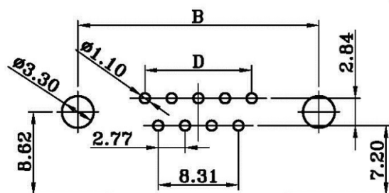
PCB LAYOUT
