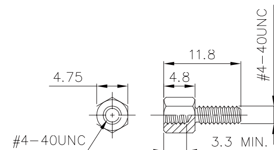
LOCKING SCREW
