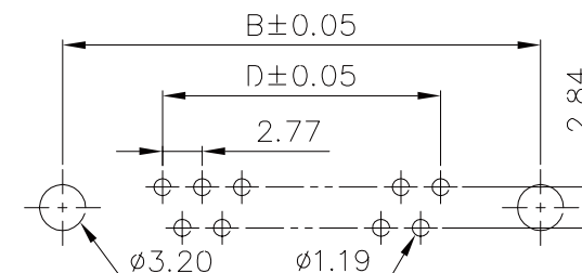
RECOMMEND P.C. BOARD LAYOUT
