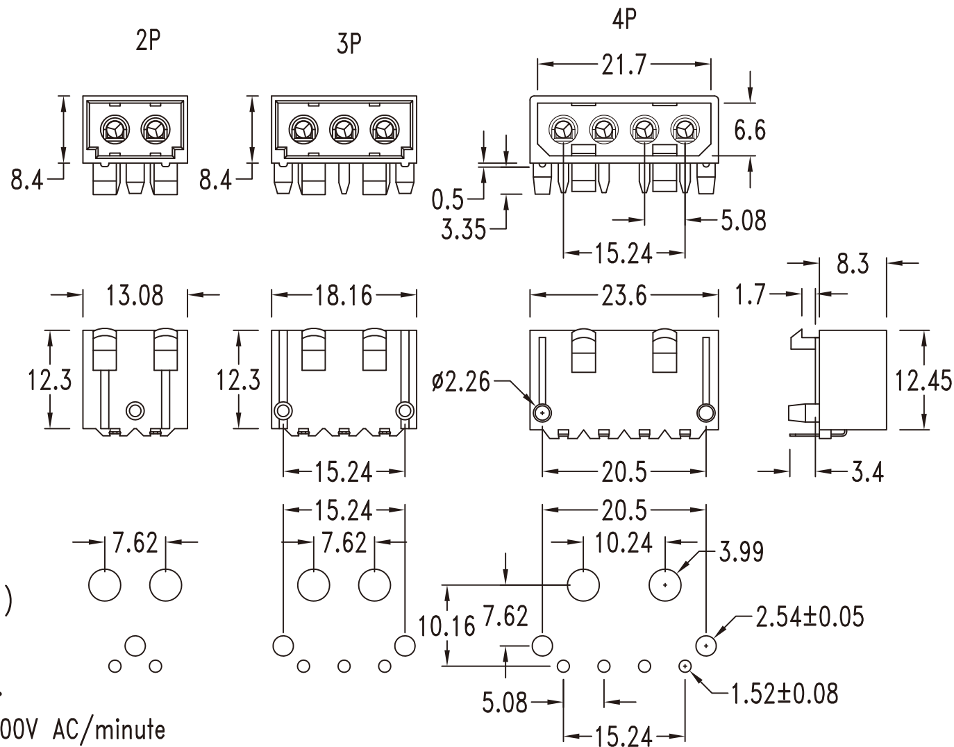
P. C. board hole dimensions
