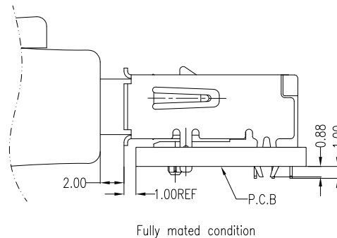
Fully mated condition
