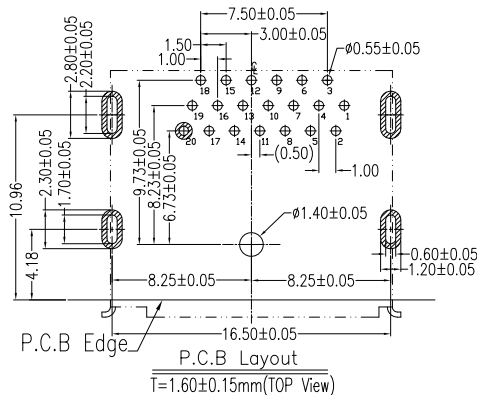
T=1.60±0.15mm(TOP View)
