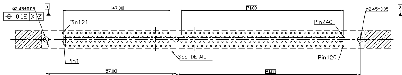
Recommend PCB Layout (Top View) Tolerances: \pm 0.05
