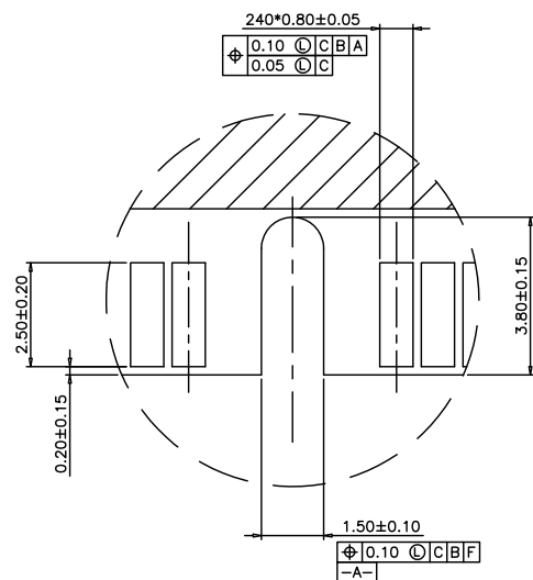
DETAIL M(5:1)
