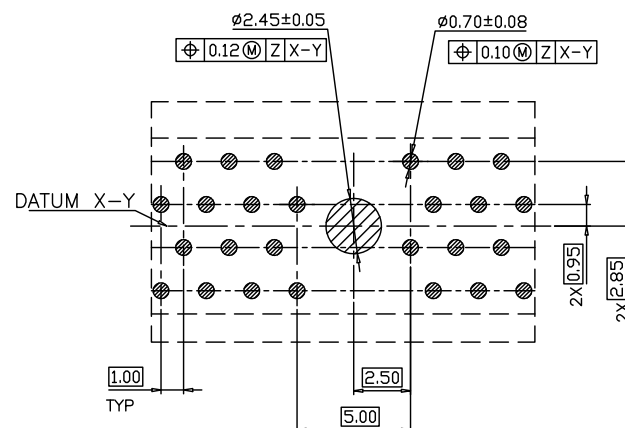
DETAIL I Option 1: Center Round Hole
