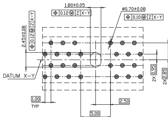
DETAIL I Option 2: Center Slot
