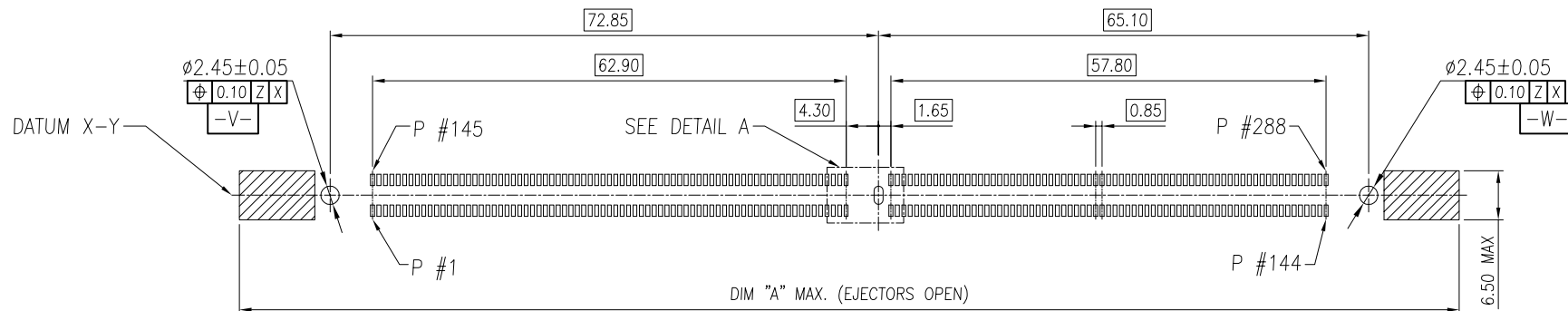
RECOMMENDED PCB LAYOUT (TOP VIEW) FOR 3 BOARDLOCKS
