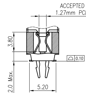
SECTION E-E SCALE 2:1
