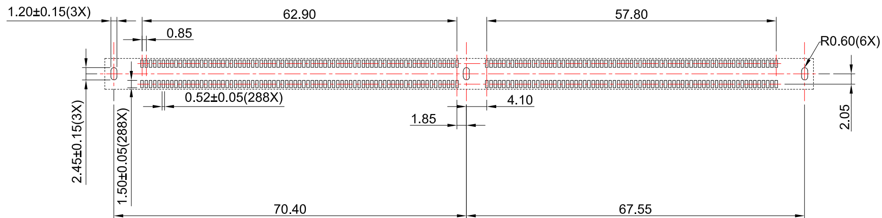
PCB LAYOUT
