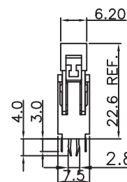
SECTION:A-A SCALE:2/1
