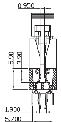
SECTION:A-A SCALE:2/1
