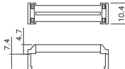
Strain Relief
