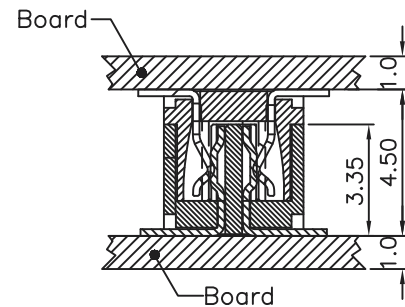
Mating Drawing (Ref.)
