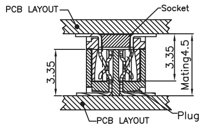
Mating Drawing (Ref.)
