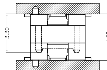
Mating Draw
