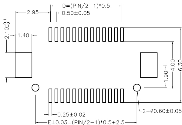
PCB MOUNTING LAYOUT
