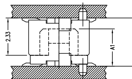
Mating Draw (Ref)
