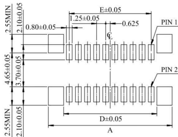
RECCOMENDED P.C.B.PATTERN LAYOUT
