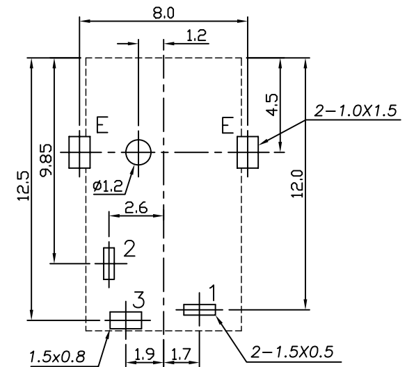
T:1.6 Dimensions of PC board holes Tolerance : \pm 0.05 Printed-Bottom view)
