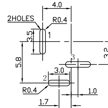
T:1.6 Dimensions of PC board holes Tolerance : \pm 0.05 (Printed-top view)
