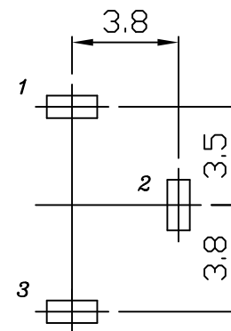
P.C.B LAYOUT ( \pm 0.1 ) (BOTTOM VIEW)
