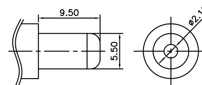
mating plug (SCALE 2:1)
