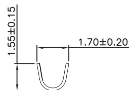
SECTIONS: B-B
