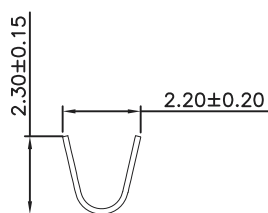
SECTIONS: A-A
