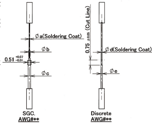
SGC. Dimension
