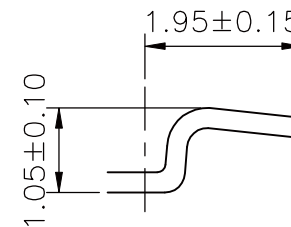
SEC:C-C
