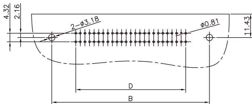
Printed Circuit Board Pattern
