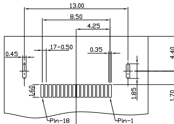
P.C BOARD LAYOUT (TOLERANCE: \pm 0.05\text{mm} )
