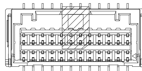
2*10P~2*14P Shape Scale 1:1
