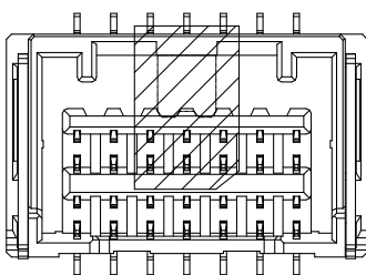
2*06P~2*09P Shape Scale 1:1
