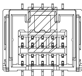
2*04P~2*05P Shape Scale 1:1
