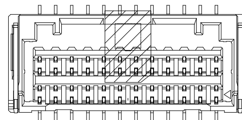
2*10P~2*14P Shape Scale 1:1
