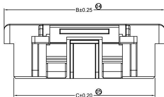
2*06P~2*14P Shape Scale 1:1
