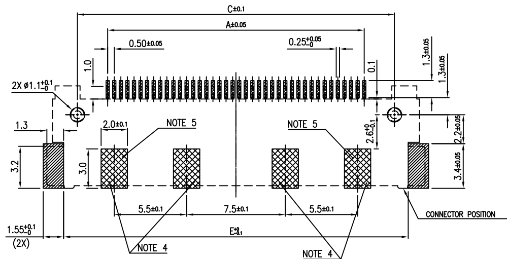
PCB PATTERN LAYOUT
