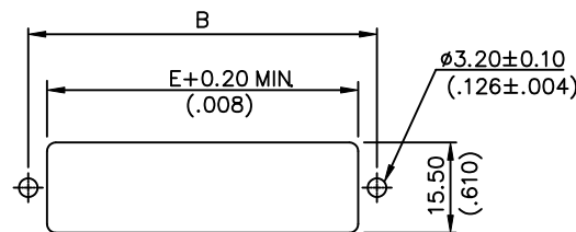
RECOMMEND FRONT MOUNT PANEL
