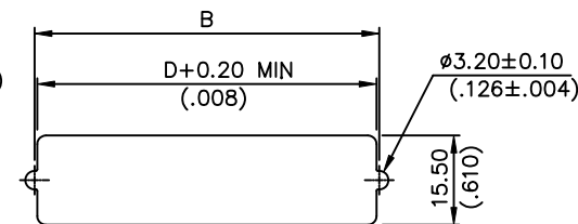
RECOMMEND REAR MOUNT PANEL
