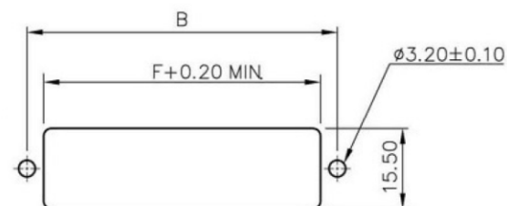
RECOMMEND FRONT MOUNT PANEL
