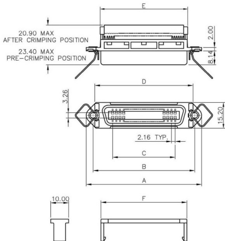
STRAIN RELIEF
