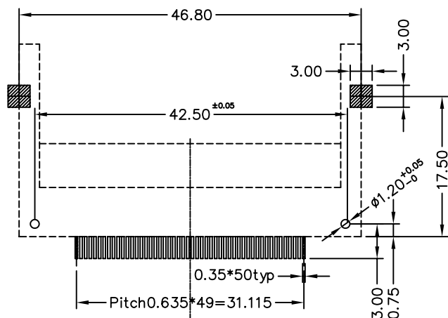
PCB Layout
