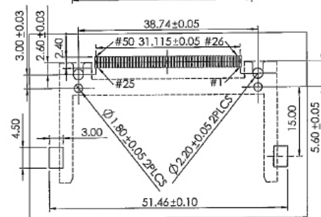
Recommended P.C.B Pattern
