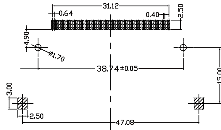
Recommended P.C.B Layout(Top Side)
