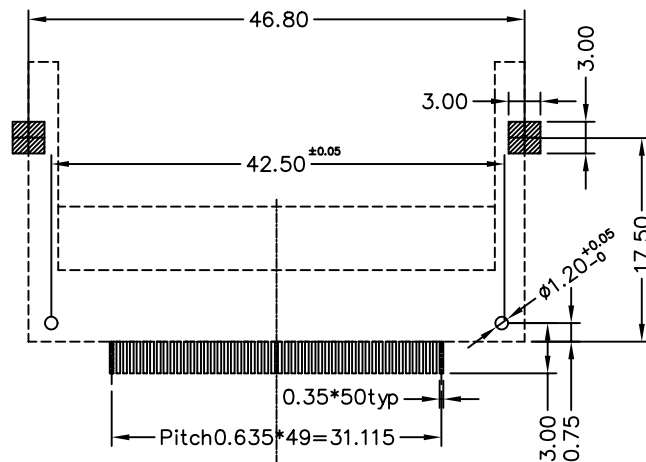
PCB Layout
