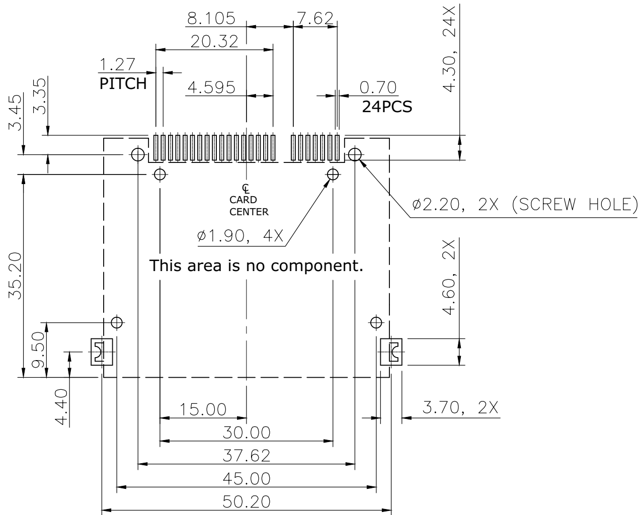
RECOMMENDED LAYOUT (TOP VIEW)
