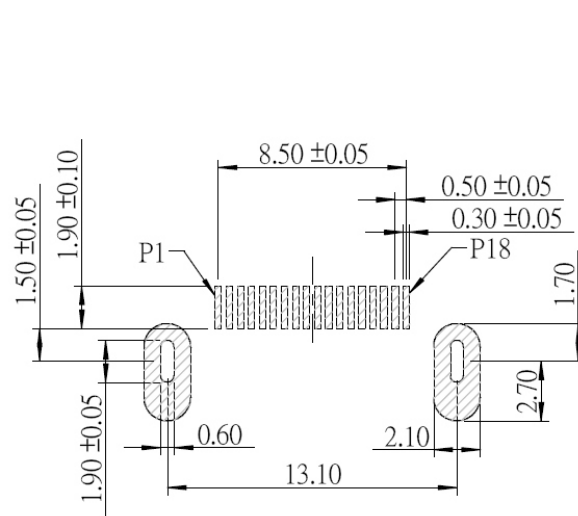
PCB Pattern
