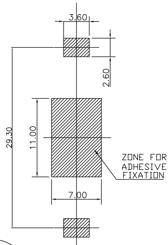
PCB LAYOUT
