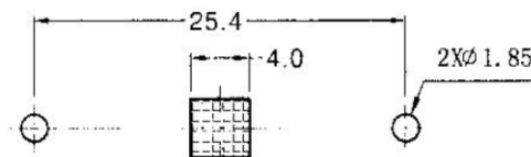
PCB Mounting layout
