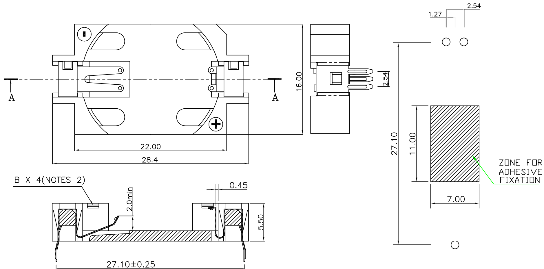
PCB LAYOUT
