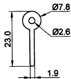
PIN
