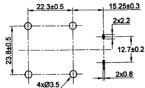
PCB/MOUNTING LAYOUT
