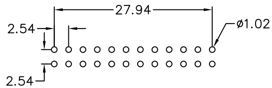
Recommended P.C.B Layout Tolerance: \pm 0.03
