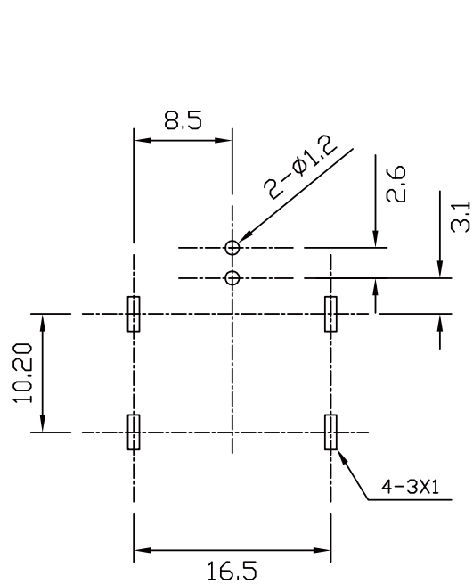
PCB LAYOUT (RECOMMENDED)
